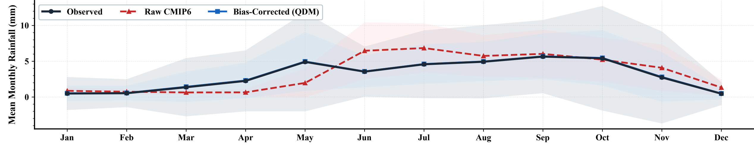
(a) Regional Mean Monthly Climatology ( 1\pm\sigma shading)
